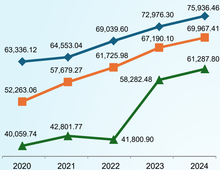
Neraca Daya (MW) Power Balance (MW) Installed Capacity Rated Capacity Peak Load
